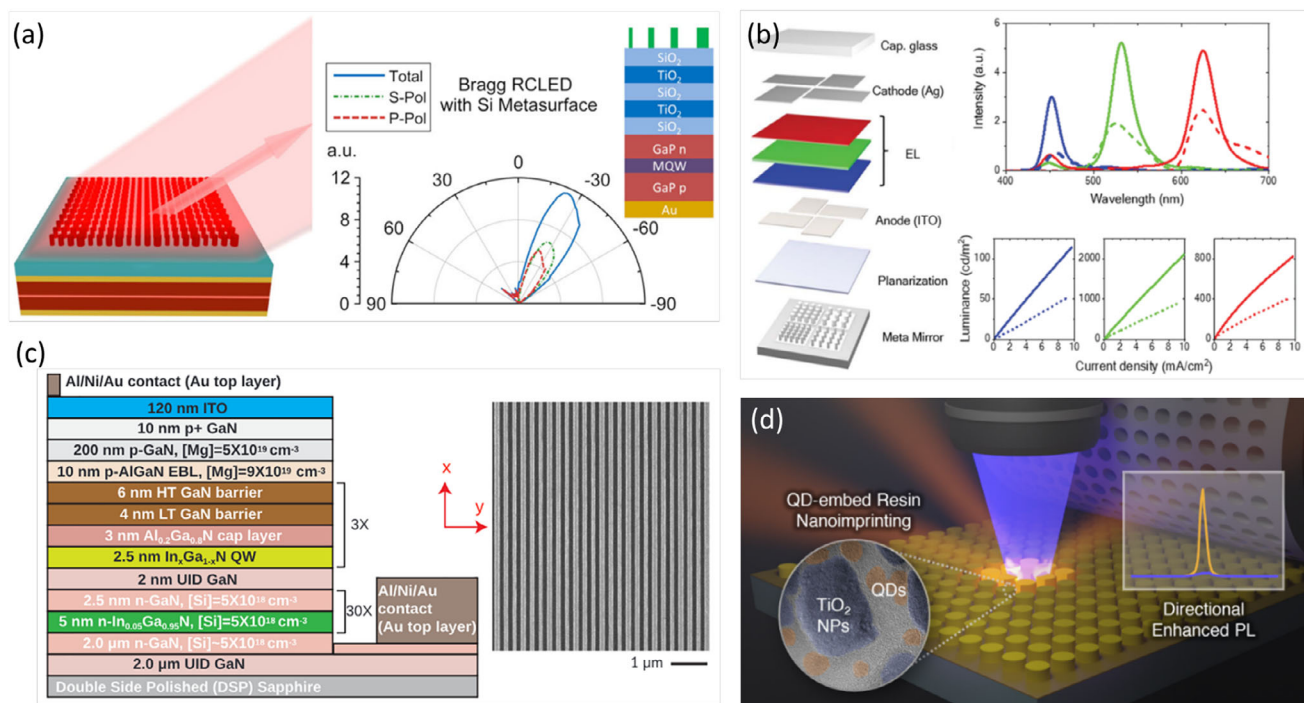
Figure 5. a) Metasurface-mediated directional electroluminescence (EL) in a LED. b) A metamirror integrated into a white-light OLED platform allows for optimal extraction of red, green, and blue light in a high-density pixel. c) A design allowing for a 1-d metasurface embedded with electroluminescent semiconductor emitters. d) Nano-imprint lithography presents a method of quickly fabricating large numbers of wide-area luminescent metasurfaces. Figures (a) adapted with permission from [80] copyright 1999-2024 John Wiley & Sons, Inc or related companies, (b) adapted with permission from [74] copyright 2024 American Association for the Advancement of Science, (c) reprinted with permission from [135] copyright 2023 American Chemical Society, (d) reprinted with permission from [136] copyright 2024 American Chemical Society.
