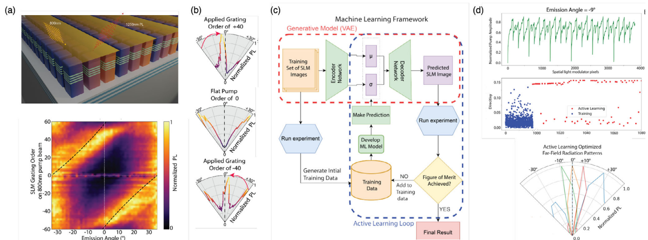
Figure 6. a) (top) Schematic of a GaAs metasurface with an imposed pump resulting in luminescence from the embedded InAs quantum dots (bottom) Luminescence across a 70° angle, by varying the grating order of the pump pattern projected on the metasurface [137] b) Examples of emission directivity for three grating order based pump patterns imposed on a GaAs metasurface c) Machine learning framework to discover pump patterns with optimal emission directivity. The framework involves a generative model (VAE) to generate arbitrary pump patterns, and Bayesian optimization to discover optimal pump patterns in the search space defined by the latent space of the trained VAE. [138] d) (top) Illustrative result, showing the optimal pump pattern found for one emission angle. (below) Luminescence obtained from using pump patterns found by the machine learning framework, across multiple emission angles. Panels (a) and (b) are adapted from [137] CC BY-NC-SA 4.0. Panels (c) and (d) are adapted from [138] CC BY-NC-SA 4.0.
