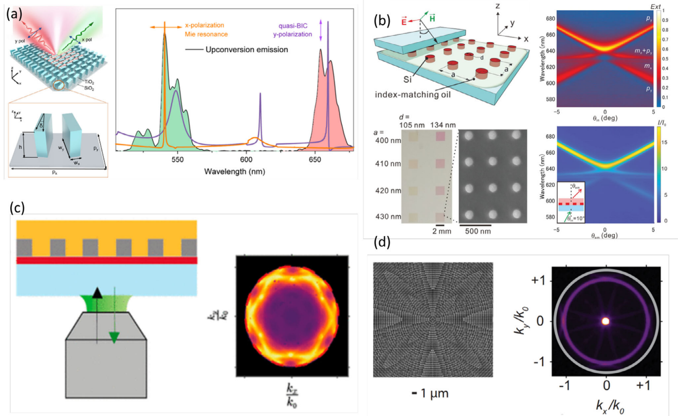
Figure 4. a) A non-uniform dielectric metasurface integrated with Lanthanide-doped up-converting nanoparticles allows for polarization-controlled enhancement of dual-band upconversion. b) Directional light emission from a uniform array of dielectric nanodisks engineered to support electric and magnetic Mie surface lattice resonances. c) A nanopatterned perovskite film (orange) yields directional photoluminescence (PL) emission. d) A meta-axicon for focusing PL, composed of semiconductor quantum well emitters embedded in nanopillars. Figures (a) adapted from [105] copyright CC-BY, (b) reprinted from [124] copyright CC-BY-NC-ND, (c) reprinted from [113] copyright CC-BY, (d) reprinted from [131] copyright CC-BY.
