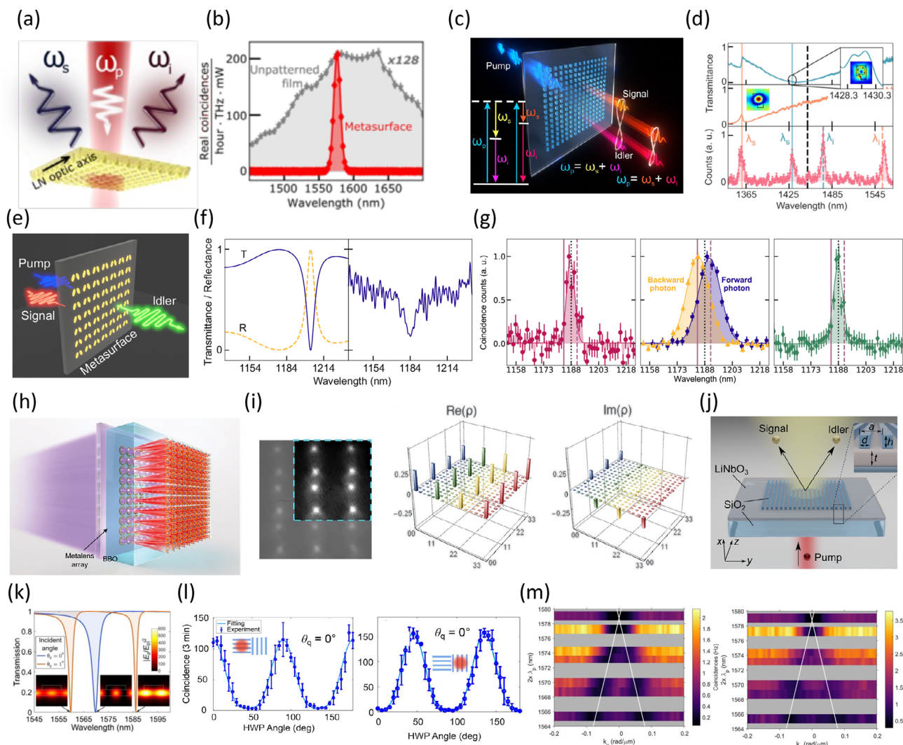
Figure 8. a–b) Backward generation of frequency-degenerate photon pairs via SPDC in a LiNbO 3 metasurface featuring Mie-type resonances. The pair generation rate is enhanced by more than two orders of magnitude compared to an unpatterned LiNbO 3 film of the same thickness. [201] c–d) Two qBICs independently generating frequency-multiplexed photon pairs in a GaAs metasurface. The electric dipole resonance at 1359.4 nm (central panel in (d)) generates a photon pair with the signal photon emitted at the resonance wavelength, while its conjugate idler photon is generated at the wavelength that conserves energy (bottom panel in (d)) given the pump laser wavelength. Likewise, a magnetic dipole resonance at 1429.4 nm (top panel in (d)) generates another photon pair at different wavelengths under the same rules. [204] e–g) SPDC in a GaP metasurfaces featuring a qBIC resonance (left panel in (f): simulated reflection and transmission spectra. Right panel in (f): measured transmission spectrum). The resonant qBIC at 1184 nm is emitted backwards, while its conjugate partner photon is emitted forwards (middle panel in (g)). For any other detection configuration, i.e., forward-forward (left-hand panel in (g)) or backward-backward (right-hand panel in (g)), the SPDC spectrum shows photon pairs only within the spectral overlap of the forward-backward configuration (middle panel in (g)). [205] h–i) Multi-SPDC generation in a BBO crystal coupled to a metalens array. The metalens focuses the pump laser in an array of 10x10 spots inside the BBO crystal. Panel (i) shows the measured density matrix for a four-dimensional entangled state. [206] j–m) Frequency-degenerate SPDC from a nonlocal metasurface. An SiO 2 metagrating supports nonlocal qBICs that enhance near fields inside a LiNbO 3 film (panel (k)). The in-plane orientation of the metagrating dictates the polarization of the emitted photon pairs (panel (l), the insets show the orientation of the metagrating). The angle of emission of frequency-degenerate photon pairs can be tuned via the pump wavelength \lambda_p in both forward-forward (left-hand panel in (m)) and forward-backward (right-hand panel in (m)) directions of emission of the signal-idler pair. [207–209] a–b) Reprinted (adapted) with permission from ref. [201]. Copyright copyright 2021, American Chemical Society. c–d) Reprinted with permission from AAAS. Copyright copyright 2022, The American Association for the Advancement of Science. e–g) Reproduced from ref. [205] with permission from the Royal Society of Chemistry. h–i) From ref. [206]. Reprinted with permission from AAAS. Copyright copyright 2020, The American Association for the Advancement of Science. j–k) From ref. [207]. Reprinted with permission from AAAS. Copyright copyright 2022, The American Association for the Advancement of Science. (l) Reprinted (adapted) with permission from ref. [208]. Copyright copyright 2023, American Chemical Society. m) Adapted from ref. [209]. CC BY 4.0.
