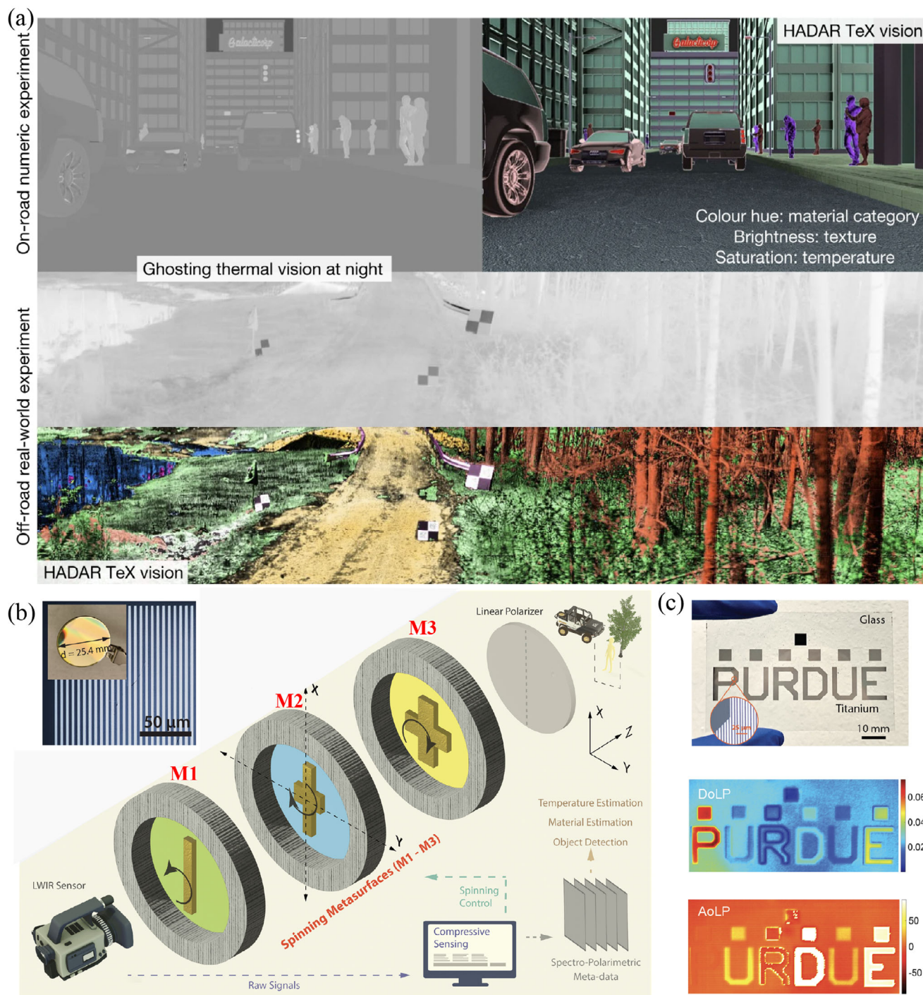
Figure 3. a) HADAR technology captures heat cubes for hyperspectral imaging, and deconstructs a textureless image using temperature, emissivity, and texture (TeX) decomposition. It is evident from TeX vision experiments that HADAR can perceive textures through complete darkness. b) Combining compressive sensing reconstruction algorithms with large-area spinning metasurfaces allows for spectrophotometric thermal imaging. c) An optical image of the imaging target with micro-structures designed to produce unique spectral and polarimetric patterns for each letter. The degree (DoLP) and angle of linear polarization (AoLP) frames reveal distinctive polarimetric signatures for each letter in the images. Figures adapted from (a) ref. [66], and (b, c) ref. [67] copyright 2024 Optica Publishing Group.
