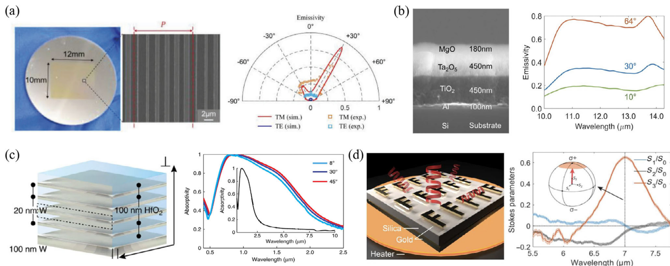
Figure 2. a) Spatially coherent thermal emission of a metagrating structure with broken mirror symmetry at wavelength 12.6 μm. b) Broadband directional thermal emission from a gradient epsilon-near-zero metamaterial. c) The absorptivity spectrum of a refractory W-HfO 2 metamaterial. d) The Stoke parameters that characterize the spin polarization of thermal emission from a symmetry-broken metasurface with F-shaped meta-atoms. Figures adapted from a) ref. [26] copyright 2023 Wiley-VCH GmbH, b) ref. [35] copyright 2021 American Association for the Advancement of Science, c) ref. [37]. CC BY 4.0., d) ref. [22] copyright 2023 American Association for the Advancement of Science.
